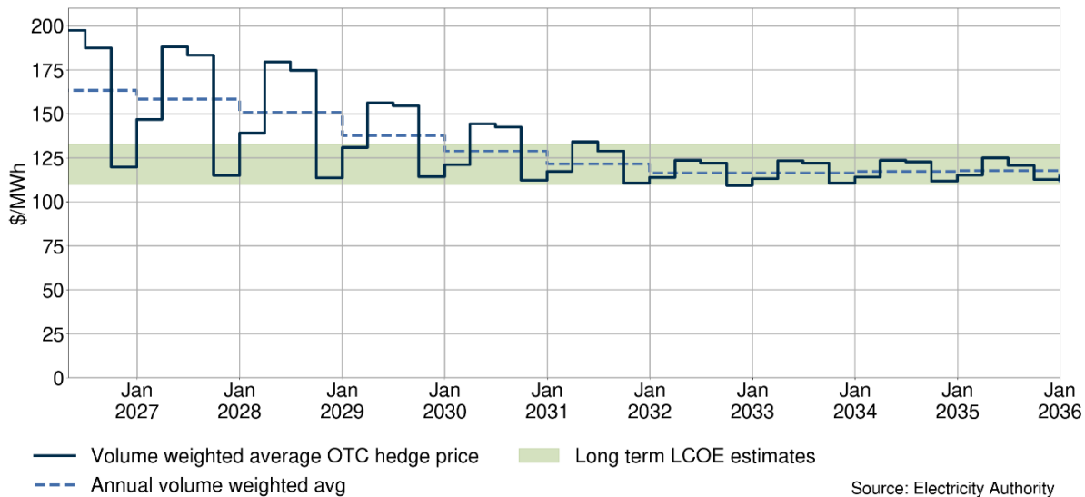
Figure 3: Baseload and 4-hourly over-the-counter (OTC) volume weighted average price, traded from May 2025, compared to levelised cost of electricity (LCOE) estimates
