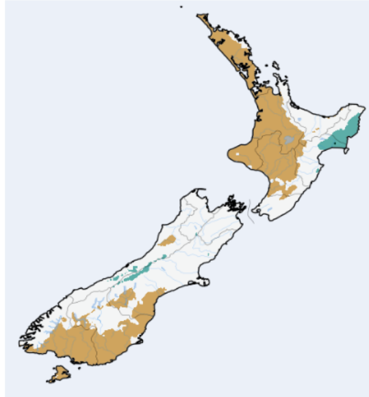
35 day rainfall anomaly (% of normal)
