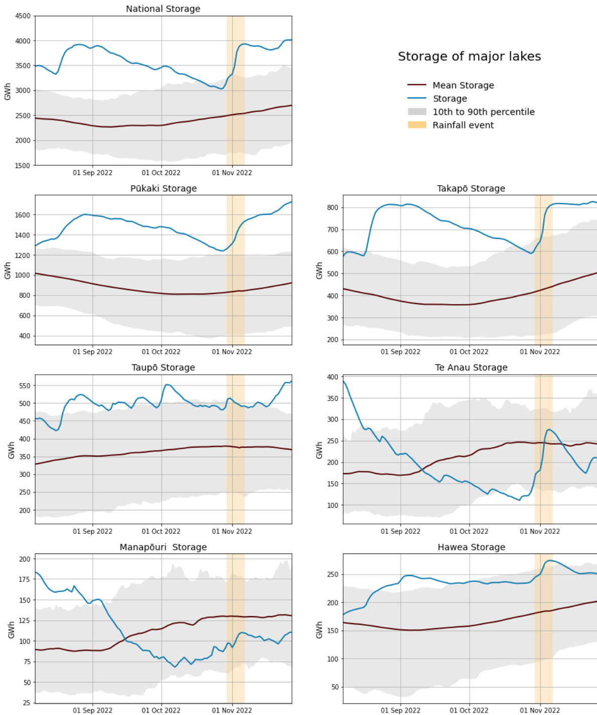
Figure 4: National hydro storage and storage at individual lakes, between 7 August and 27 November 2022, alongside each respective historic mean and 10th and 90th percentiles of historic storage levels
