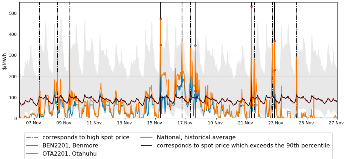
Figure 1: Half-hourly wholesale spot prices at Benmore and Ōtāhuhu between 6-27 November 2022
