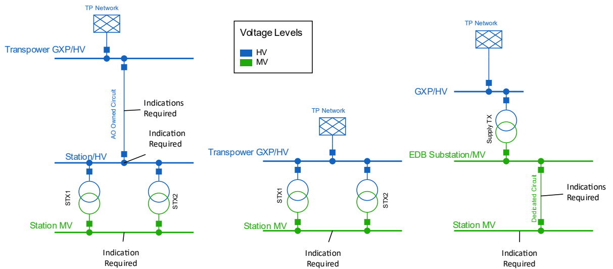
Figure A1: Typical configuration of different possible network connections with required circuit and busbar indications marked
