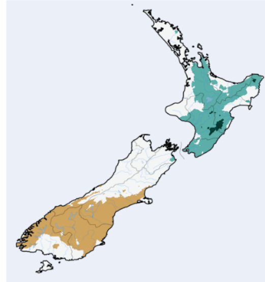
35 day rainfall anomaly (% of normal)
