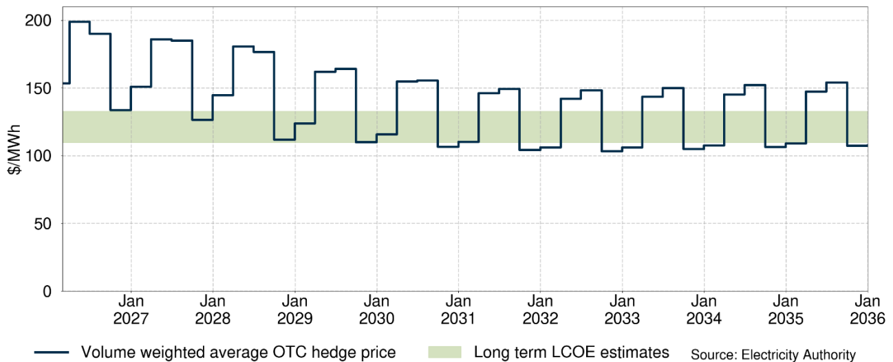
Figure 4: Baseload and 4-hourly over-the-counter (OTC) volume weighted average price, traded from 2025, compared to levelised cost of electricity (LCOE) estimates
