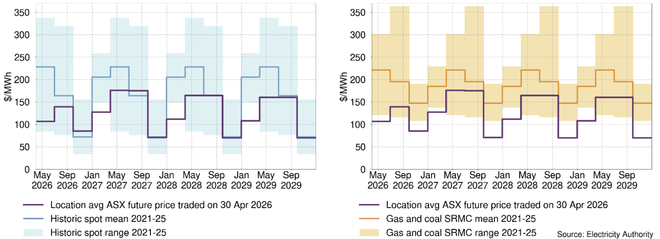
Figure 2: ASX future price (average of Ōtāhuhu and Benmore) compared to historic average spot prices and historic average gas and coal short run marginal costs (SRMCs)
